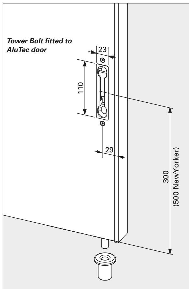
Tower bolt on CS AluTec door.
